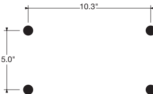
Mounting Pattern
